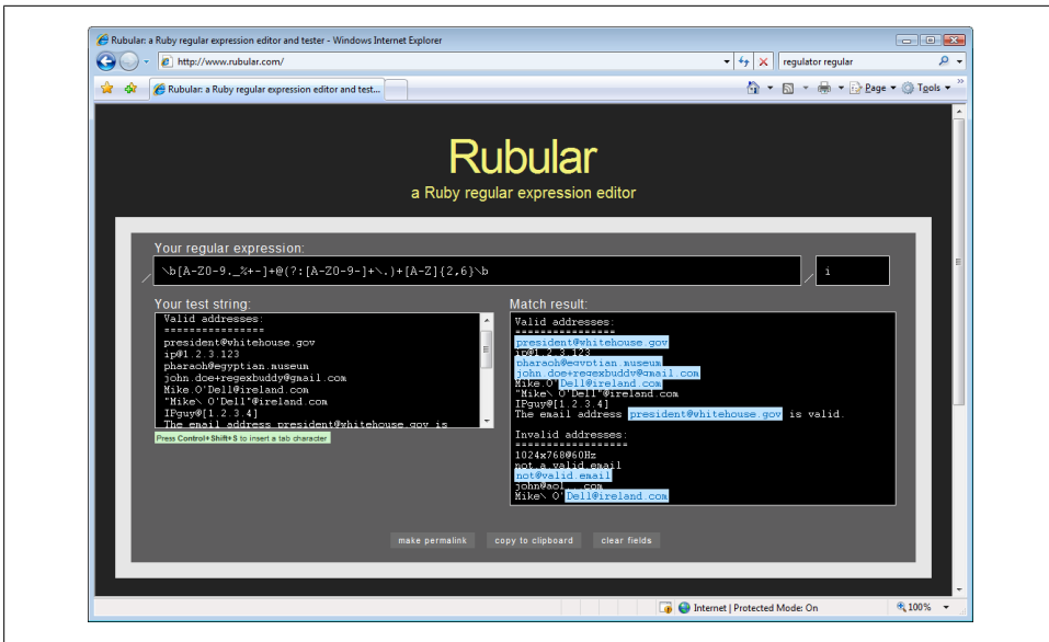
Figure 1-7. Rubular
