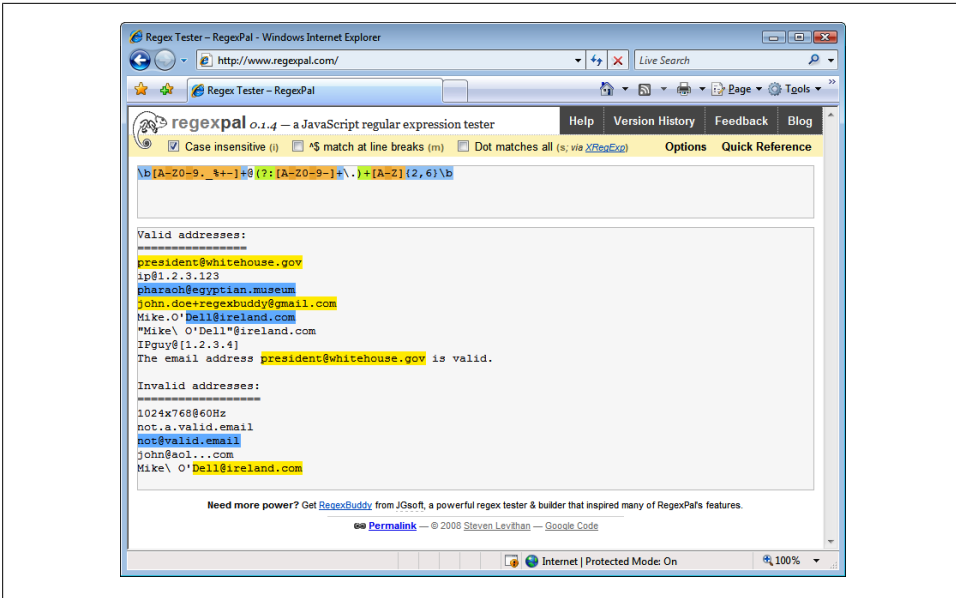
Figure 1-2. Regexpal
