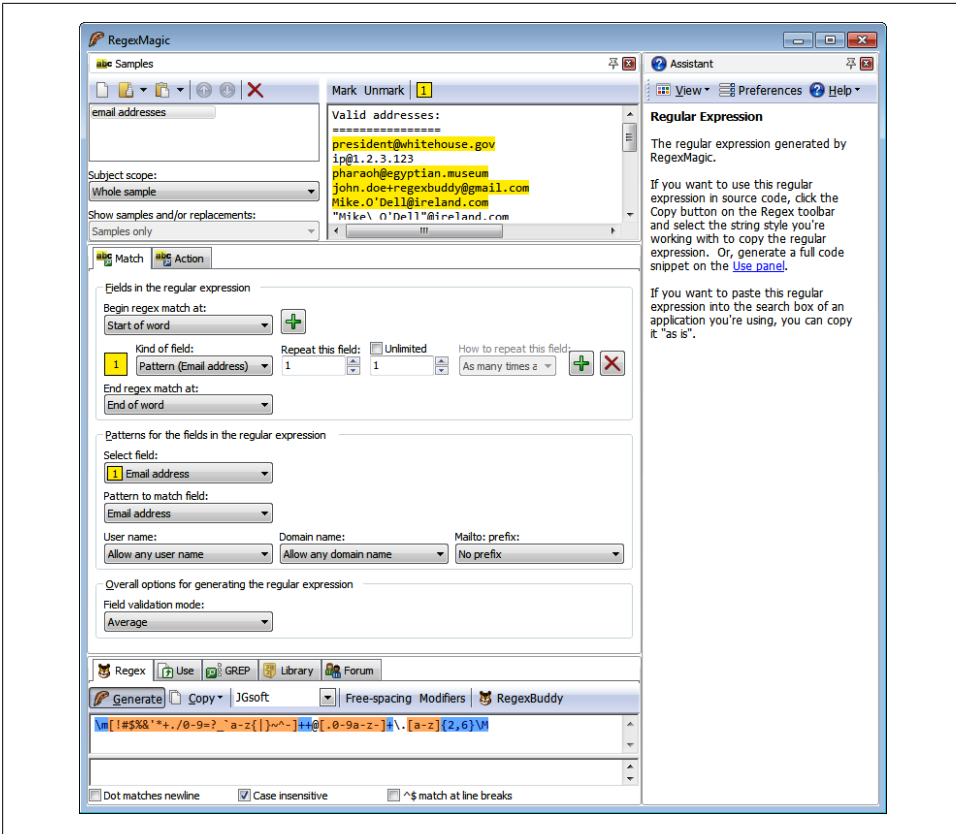
Figure 1-3. RegexMagic
